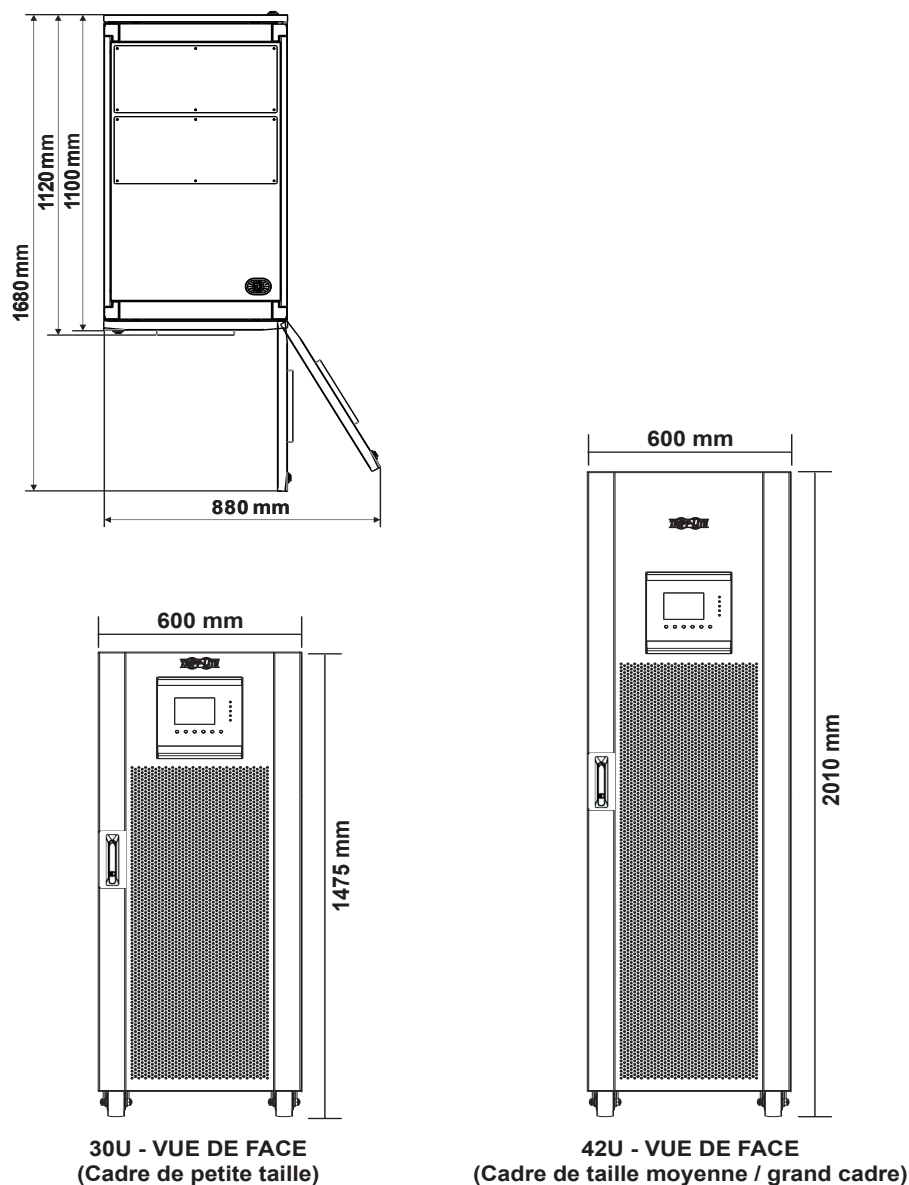
Figure 3-1 : Dimensions
