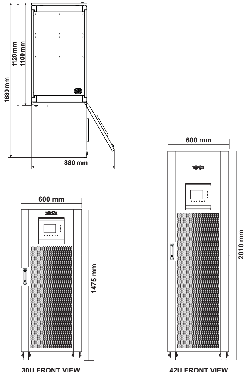
Figure 3-1: Dimensions
