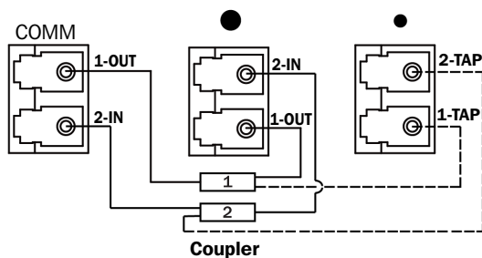
LC to LC TAP port mapping
