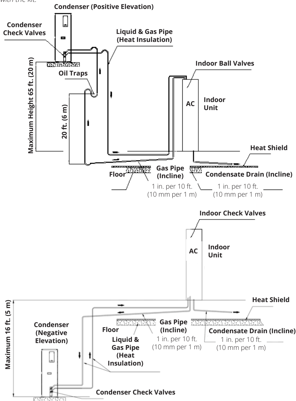
Figure 4-1: Piping Examples
