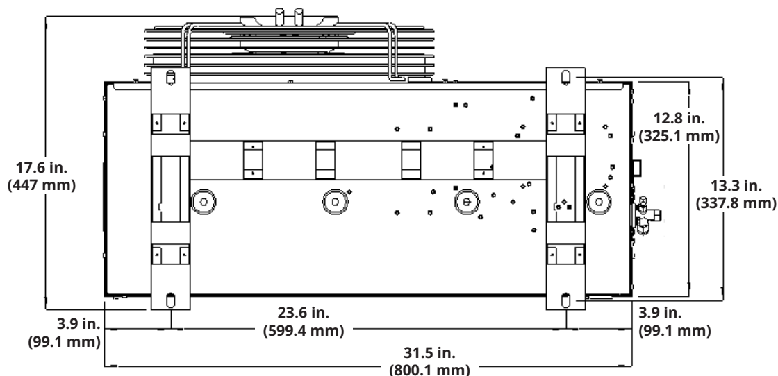
Figure 3-5: Condenser Mounting Interface (bottom view looking up), SRCOOLDXRW12
