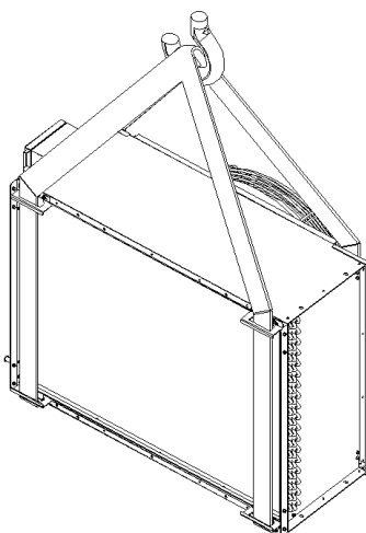
Figure 3-2: Example of Lifting the Condenser
